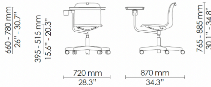
Side chair - polypropylene
