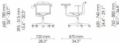
Armchair - polypropylene
